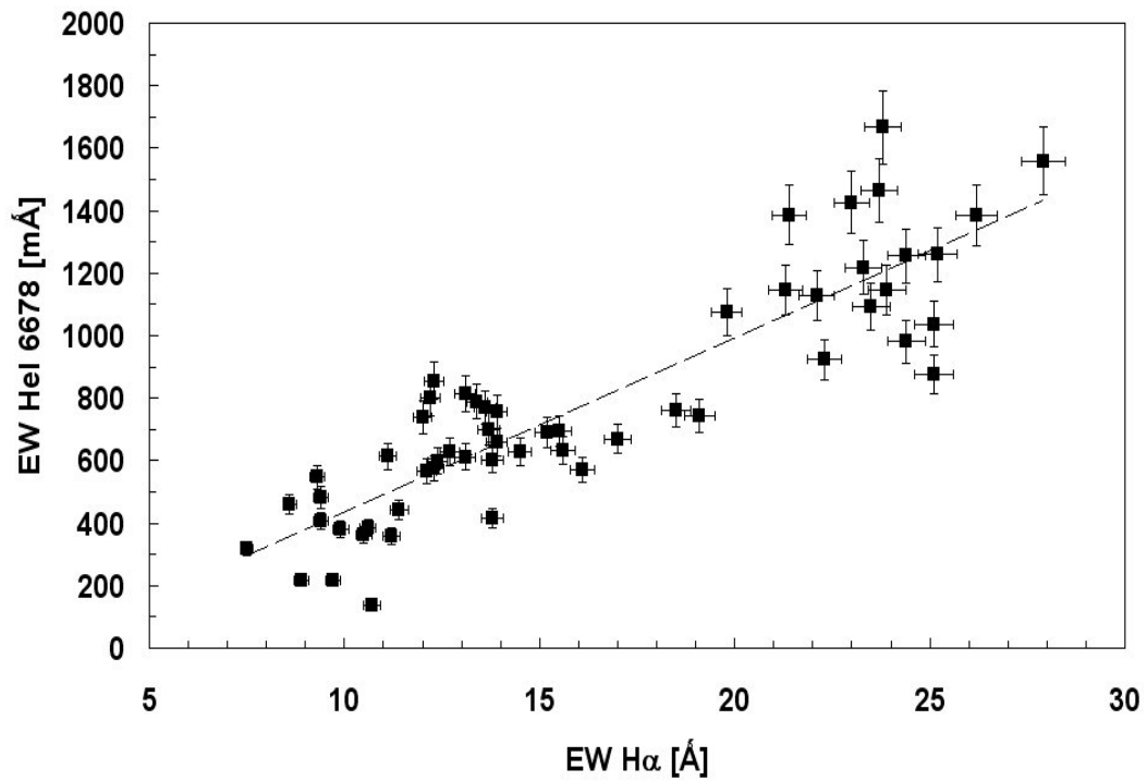
Fig. 1: Correlation between equivalent width of HeI \lambda 6678 Å and H \alpha since 04/2005
